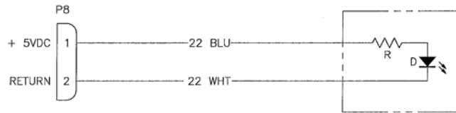
WIRING DIAGRAM
